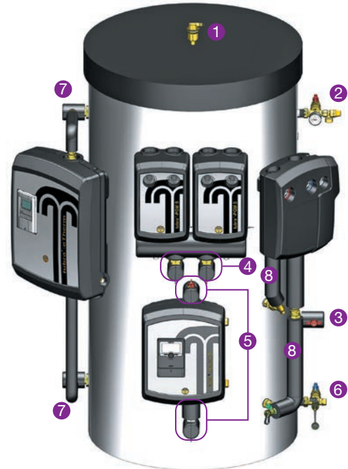
5 Frischwasserstation: nemux Fresh water station tubra® -Eckkugelhahn Set - corner ball valve set ÜWM G1 - G1 AG
